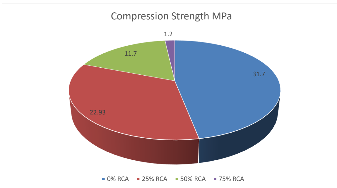
Graph 2. 7-Day Concrete Compressive Strength Comparison (MPa)
