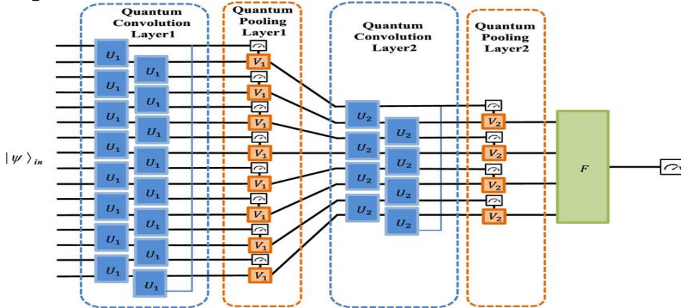
Figure 1. Quantum Convolution and Pooling Framework of the Hybrid Quantum Duplet-CNN Model.
