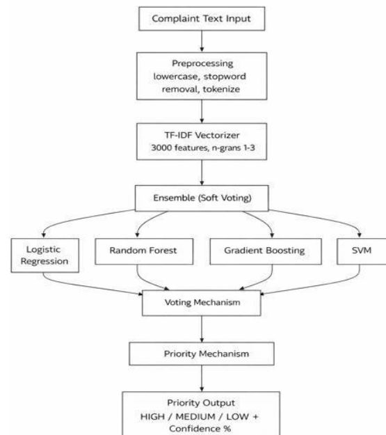
Fig. 5. ML Pipeline for Complaint Priority Classification
