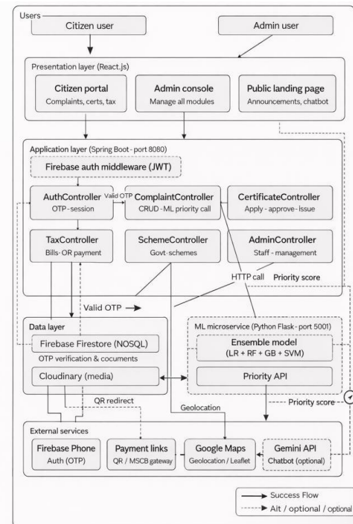
Fig. 1. Layered System Architecture of DigiGram showing Client, Backend, ML Microservice, and Data Layers.
