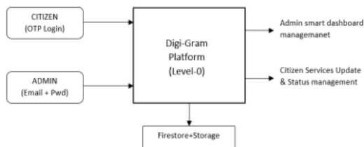
Fig. 2. DFD Level-0 (Context Diagram) — DigiGram Platform
