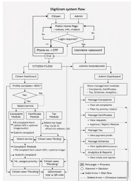
Fig. 4. Citizen Complaint Submission Flowchart — From Login to Resolution
