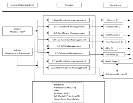
Fig. 3. DFD Level-1 Decomposed Process View of DigiGram Modules
