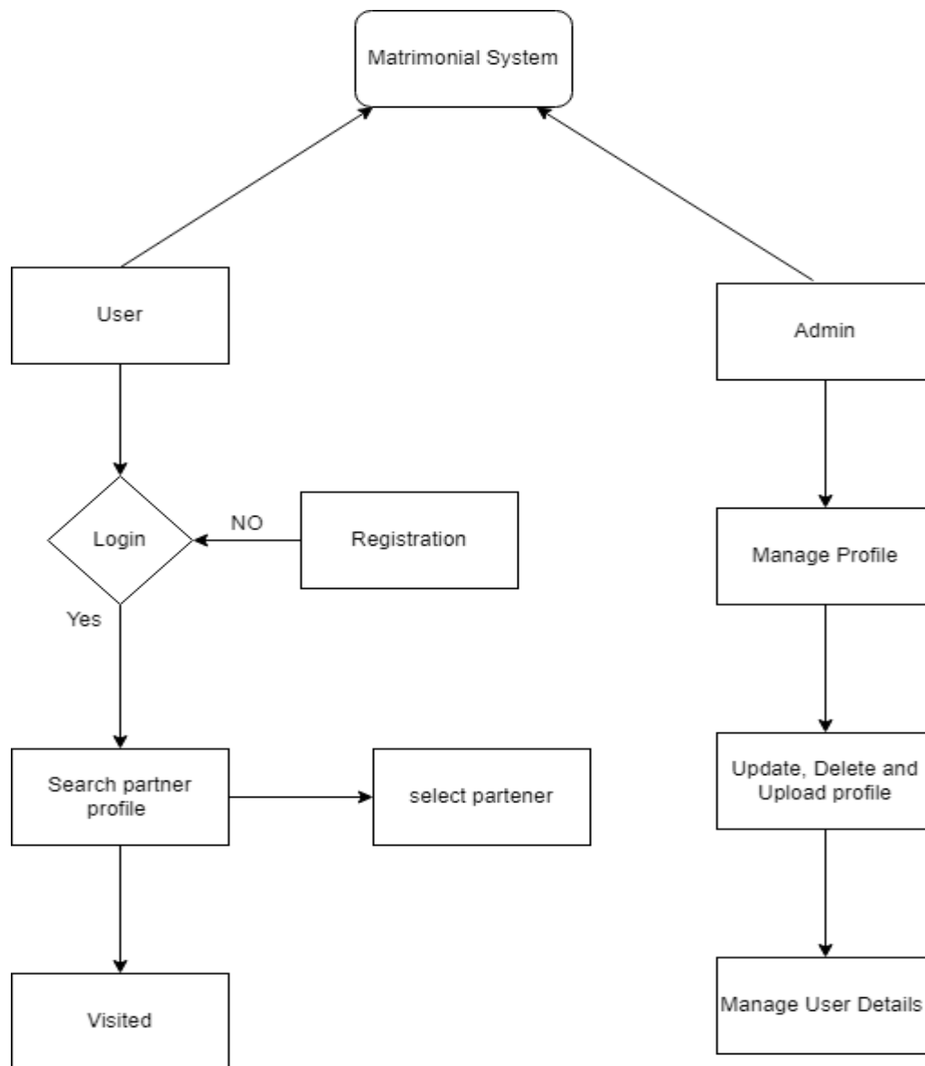
Fig 1:-System Architecture
