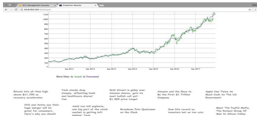
Fig 4. The Predicted Stock Price for tomorrow. The figure also shows the plot of the actual stock price against the predictions
