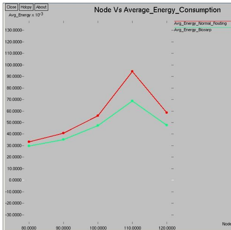
Fig.6 Energy Consumption
