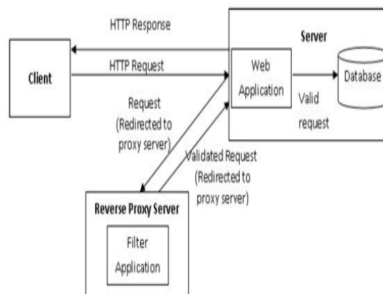
Fig 1. Proposed Workflow
