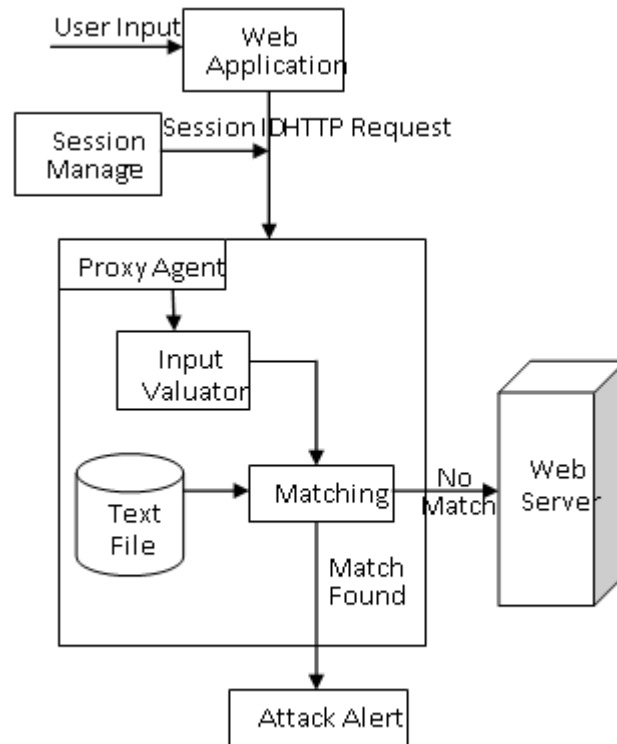
Fig. 3 Block diagram of Query detector.
