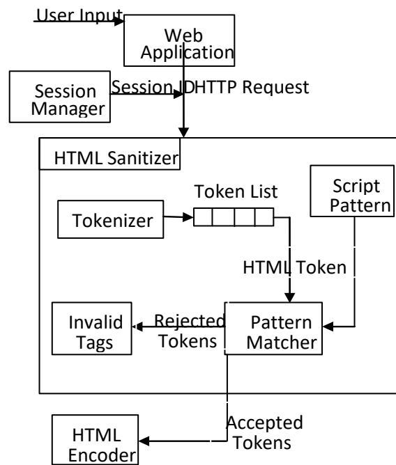
Fig. 2 Block diagram of Script detector
