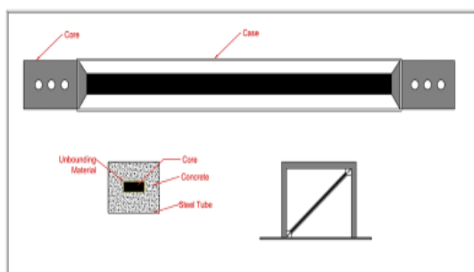
Fig 2: Schematic representation of a buckling restrained brace
