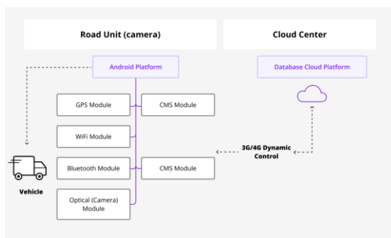
Fig 1. Real time Video Based Surveillance System
