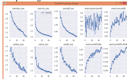
Fig 3. Training Graph
