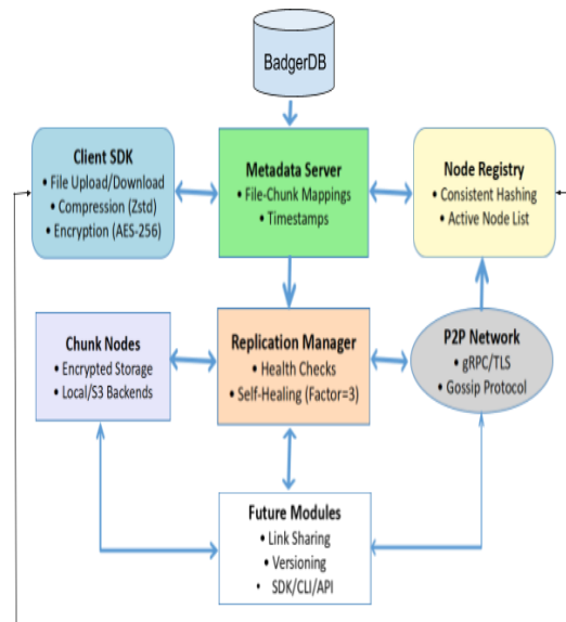
Fig 1: Block Diagram of DisktroByte
