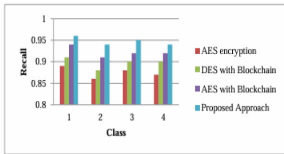
(c) Recall
