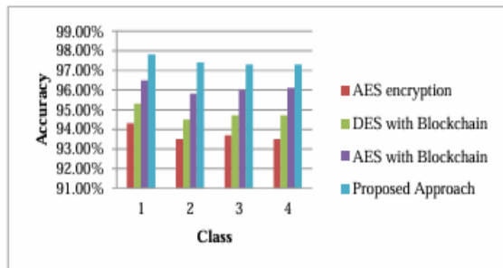
(a) Accuracy
