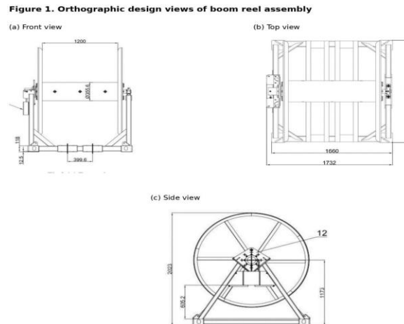
Fig. 1. Orthographic design views of the proposed boom reel assembly showing front, top, and side views.
