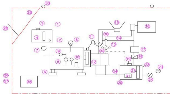
Fig. 2. Hydraulic powerpack circuit diagram used for controlled operation of the boom reel system.
