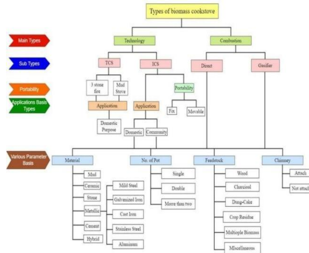
Fig. 1. Types of Biomass Cook Stoves
