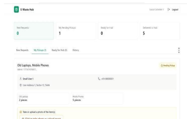
Fig. 4. Collector Dashboard
