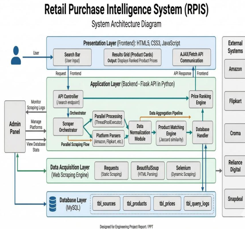
Fig. 1. System Architecture of the Retail Purchase Intelligence System (RPIS)
