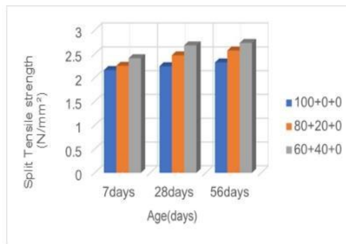
Graph 2. Split Tensile strength variation in different mixes with 0% glass fiber
