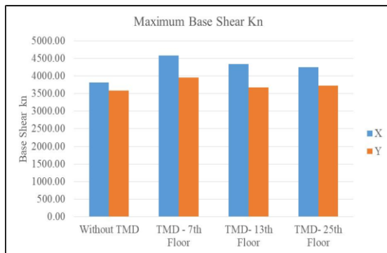
Graph 3. Maximum Base Shear
