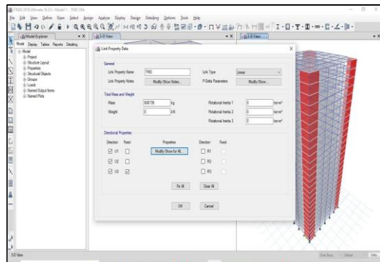
Fig 3: TMD Define in ETABS
