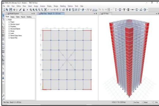
Fig 2: Modelling in ETABS
