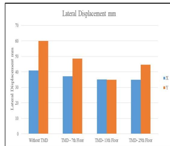
Graph 2. Lateral Displacement mm
