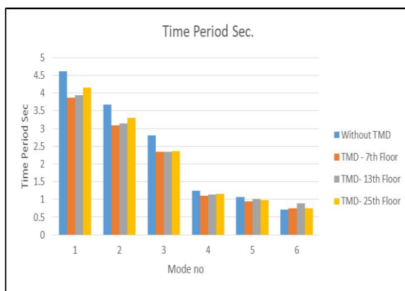
Graph 1: Time Period Sec.
