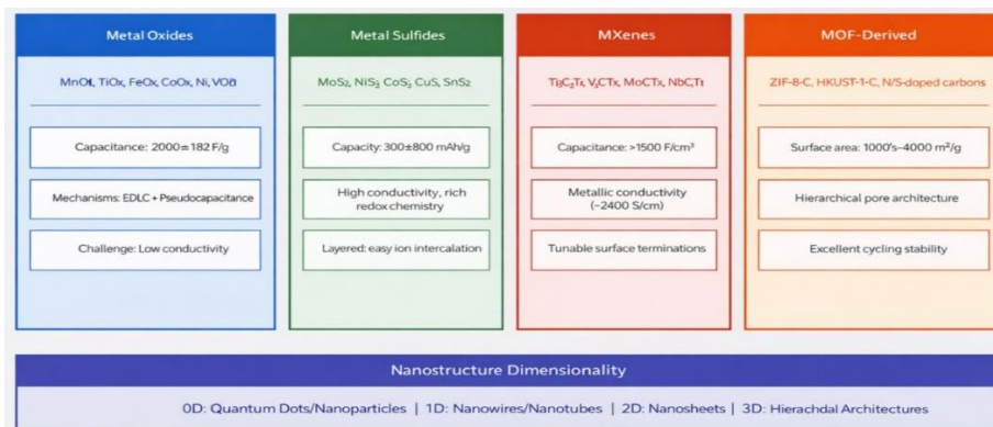
Figure 3: Overview of key nanostructured inorganic material systems for energy storage, comparing crystal structure features, charge storage mechanisms, and representative electrochemical performance metrics.
