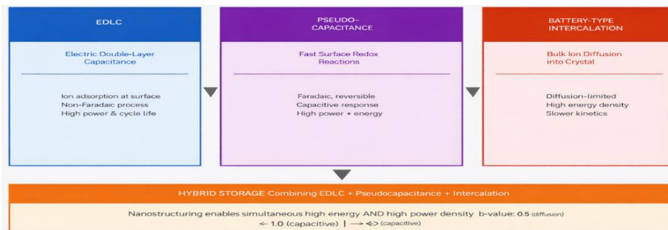
Figure 2: Comparative schematic of electrochemical charge storage mechanisms in nanostructured inorganic materials, illustrating the progression from purely capacitive (EDLC) to diffusion-limited (battery-type) behavior and the role of nanoscale engineering in mechanism hybridization.
