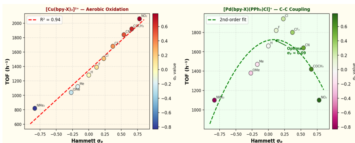
Figure 2. Electronic tuning of catalytic TOF via Hammett substituent constants for Cu(II) and Pd(II) complexes
