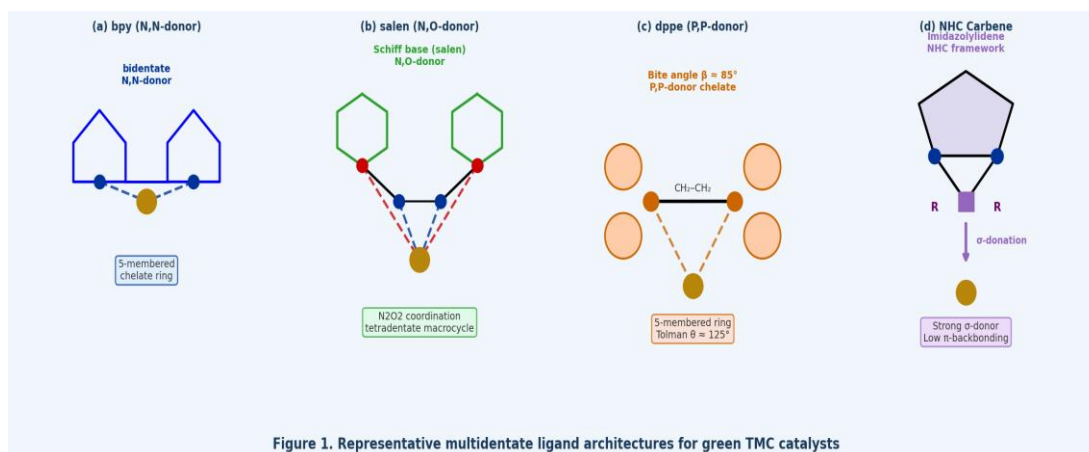
Figure 1. Representative multidentate ligand architectures for green TMC catalysts
