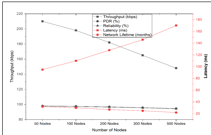
Figure 7: Scalability and Reliability Performance Analysis of Proposed WSN-AI System
