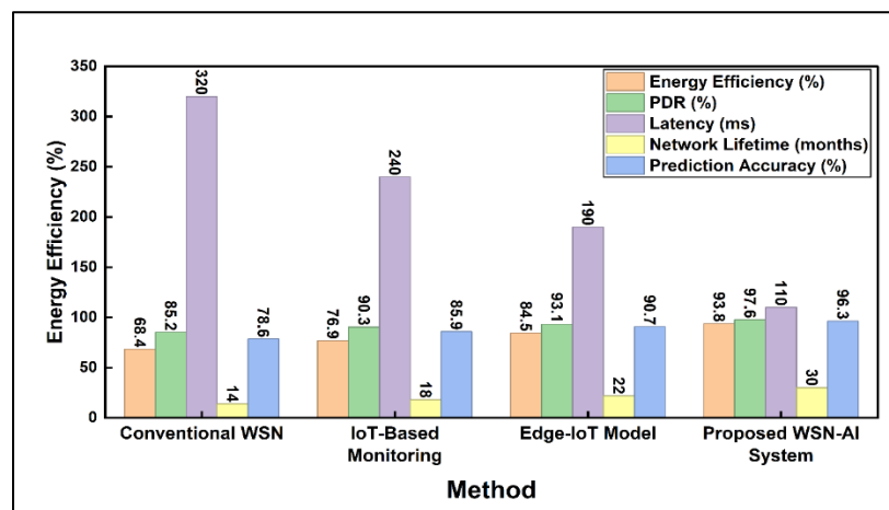
Fig. 5. Comparative Performance Evaluation of WSN Monitoring Approaches
