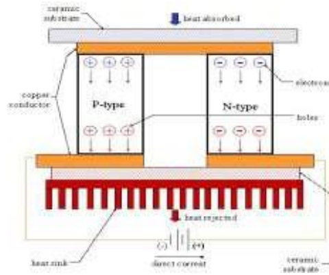
Fig 2. Principle of TEC
