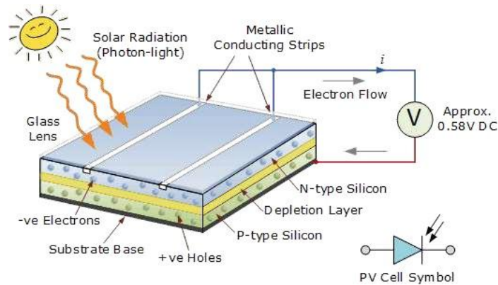
Fig 1. working of pv cell
