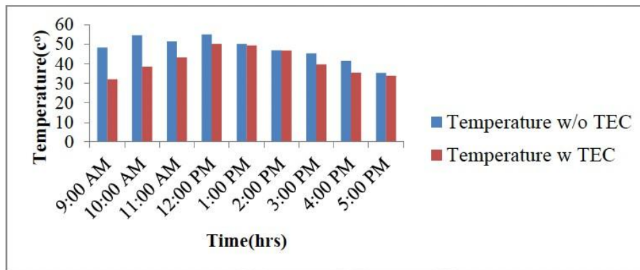
Fig 4. Comparison of Temperature
