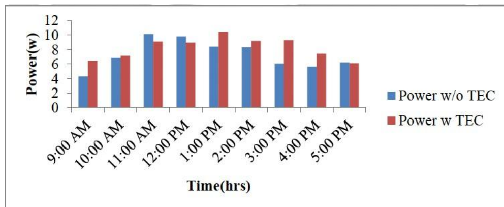
Fig 5. Effect of Thermoelectric Module on Solar Panel Power Generation
