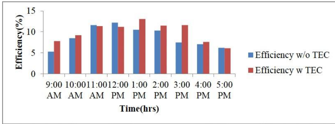
Fig 5. Efficiency Vs Time curve
