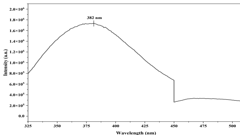
Fig. 5. Photoluminescence spectra of Phyto-Produced ZnO nanoparticles
