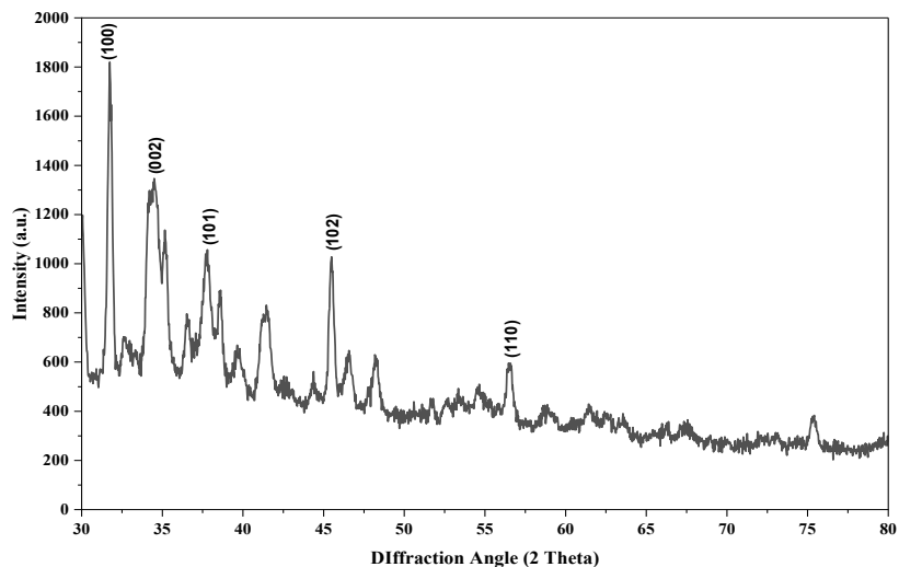
Fig. 3. XRD analysis of Eco-produced ZnO nanoparticles
