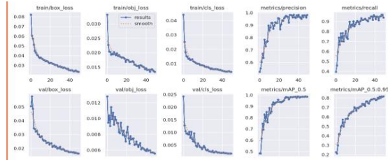
Fig 3:Yolov5 Preformance Graph
