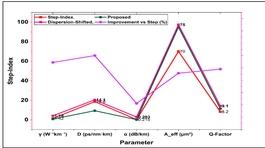
Figure 7: Comparative Performance Improvement of Proposed Fiber over Conventional Fiber Designs
