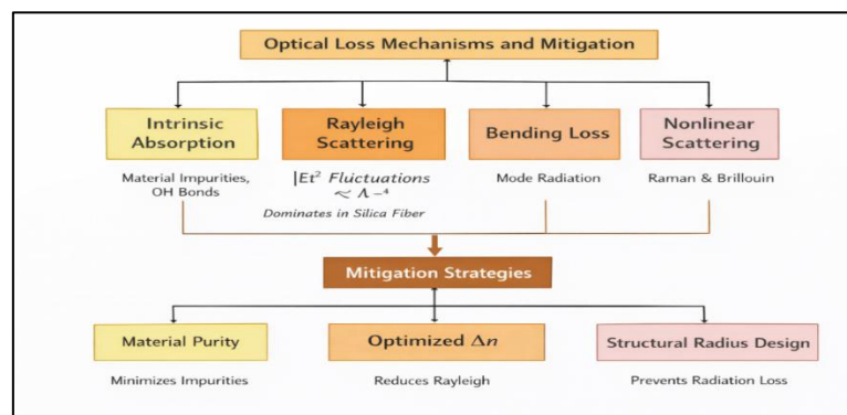
Figure 3: Optical Loss Mechanisms and Mitigation Strategies in High-Speed Optical Fiber Transmission
