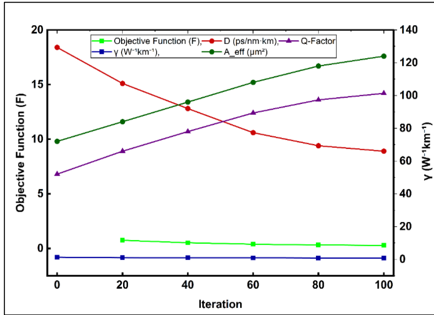
Figure 4: Convergence Behaviour of Multiphysics Co-Optimization Parameters during Iterative Optimization
