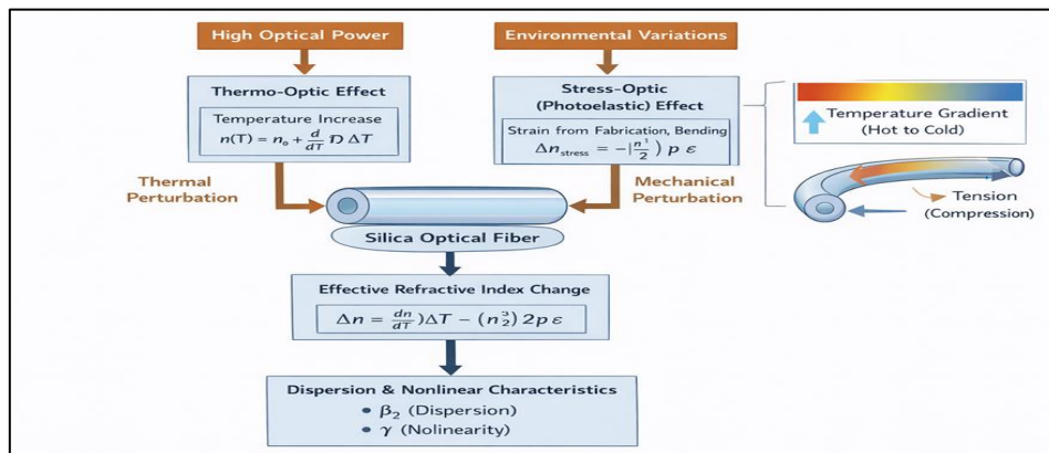
Figure 2: Thermo-Optic and Stress-Optic Coupled Multiphysics Interaction in Optical Fiber Transmission
